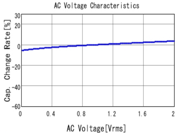
GCM32ER71E106KA57 C-AC Voltage capchange, DCOV, 25.0d
