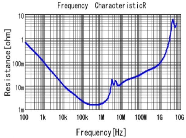
GCM32ER71E106KA57 R DCOV, 25degC
