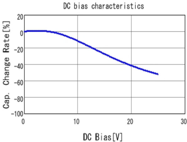
GCM32ER71E106KA57 C-DC bias capchange, 25.0degC, AC1.
