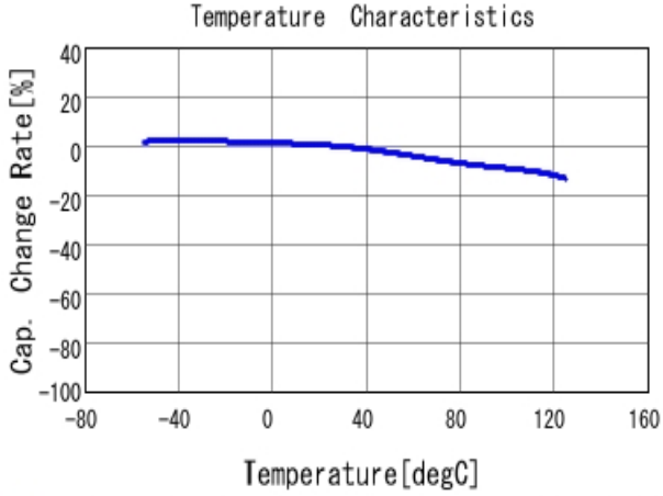
■ GCM32ER71E106KA57 C-Temp. capchange, DC0.0V, AC1.0V rm
