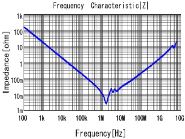
GCM32ER71E106KA57 |Z| DCOV, 25degC
