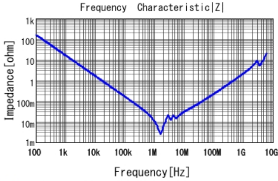
GCM32EC71H106KA03 |Z| DCOV, 25degC
