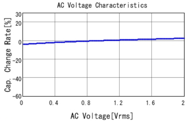
GCM32EC71H106KA03 C-AC Voltage capchange, DCOV, 25.0d
