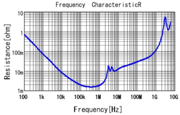
GCM32EC71H106KA03 R DCOV, 25degC
