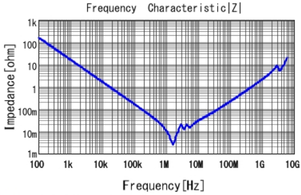
GCM32EC71H106KA03 |Z| DCOV, 25degC
