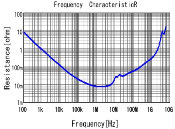
GCM31MR71H105KA55 R DCOV, 25degC
