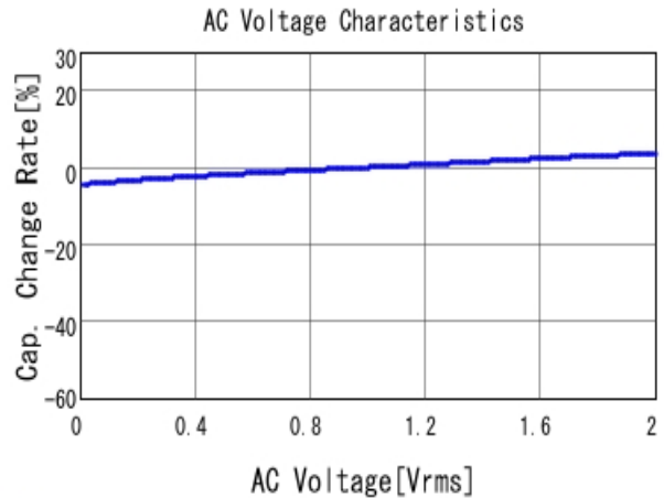
GCM31MR71H105KA55 C-AC Voltage capchange, DCOV, 25.0d
