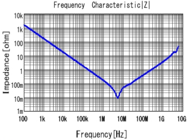
GCM31MR71H105KA55 |Z| DCOV, 25degC
