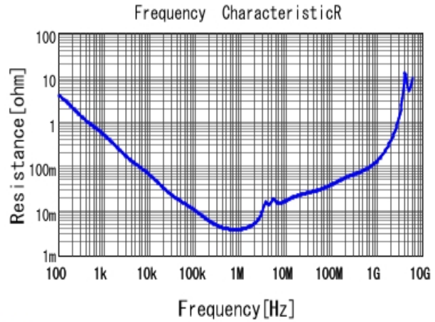
GCM31CR71C106KA64 R DCOV, 25degC
