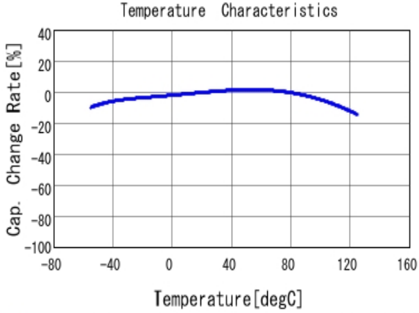
■ GCM31CR71C106KA64 C-Temp. capchange, DC0.0V, AC1.0V rm
