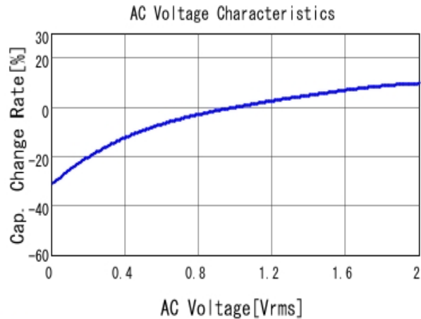
GCM31CR71C106KA64 C-AC Voltage capchange, DCOV, 25.0d
