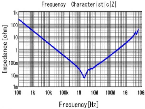
GCM31CR71C106KA64 |Z| DCOV, 25degC
