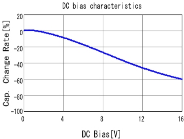
GCM31CR71C106KA64 C-DC bias capchange, 25.0degC, AC1.
