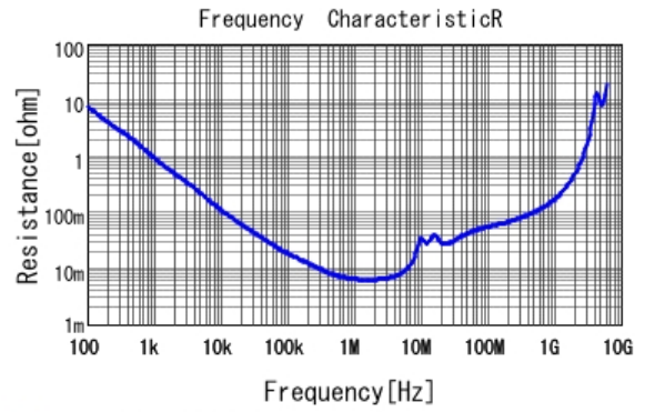
GCM31CL81H105KA55 R DCOV, 25degC
