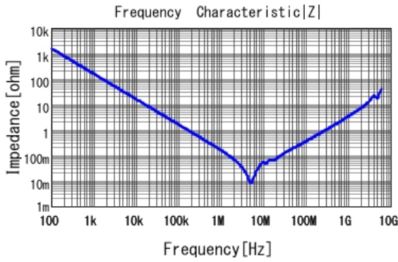
GCM31CL81H105KA55 |Z| DCOV, 25degC
