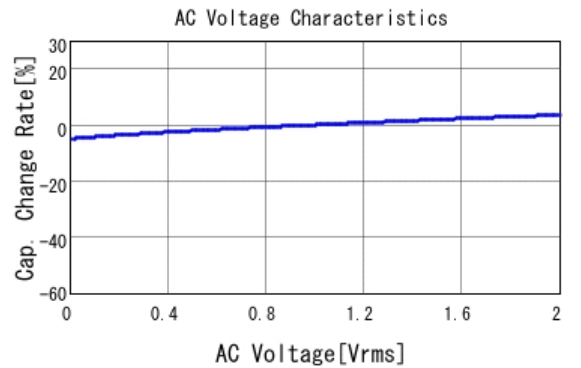
GCM31CC72A225KE02 C-AC Voltage capchange, DC0V, 25.0d
