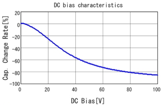
GCM31CC72A225KE02 C-DC bias capchange, 25.0degC, AC1.
