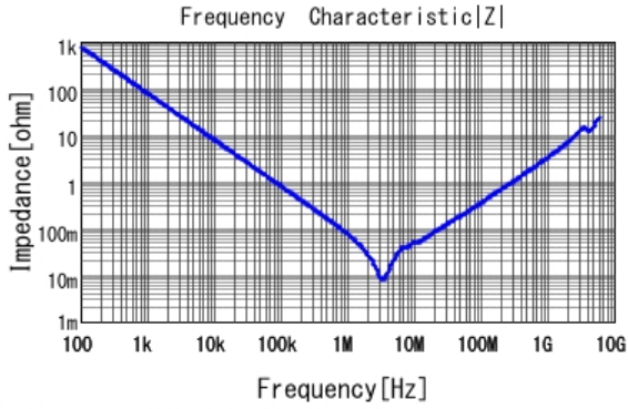
GCM31CC72A225KE02 |Z| DC0V, 25degC
