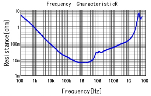
GCM31CC72A225KE02 R DC0V, 25degC
