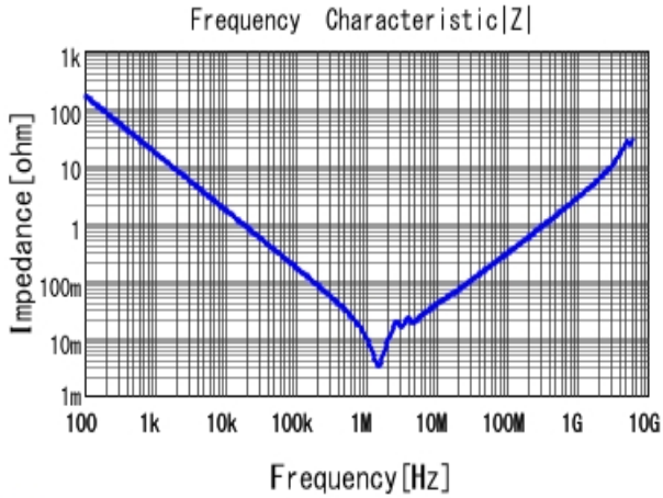
GCM31CC71E106KA03 |Z| DCOV, 25degC
