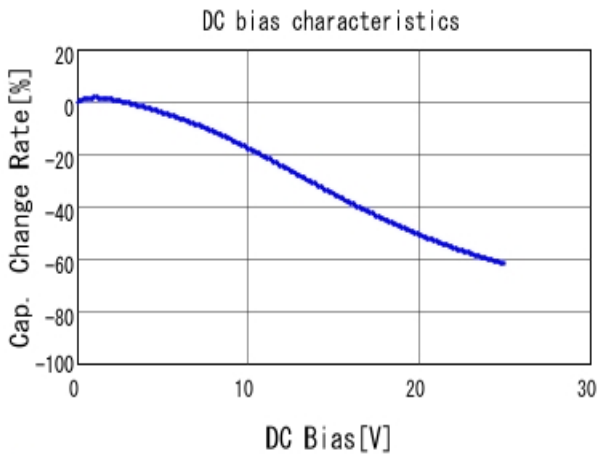
GCM31CC71E106KA03 C-DC bias capchange, 25.0degC, AC1.
