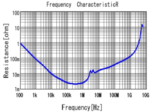
GCM31CC71E106KA03 R DCOV, 25degC
