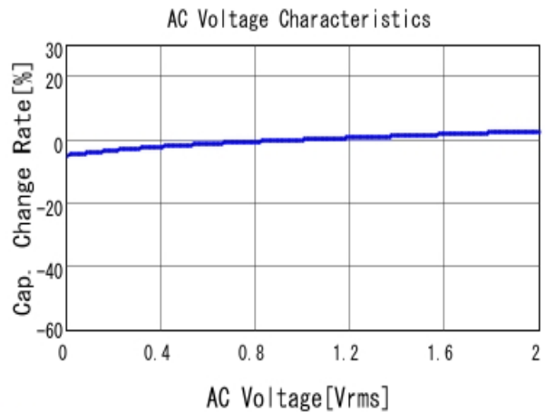
GCM31CC71E106KA03 C-AC Voltage capchange, DCOV, 25.0d
