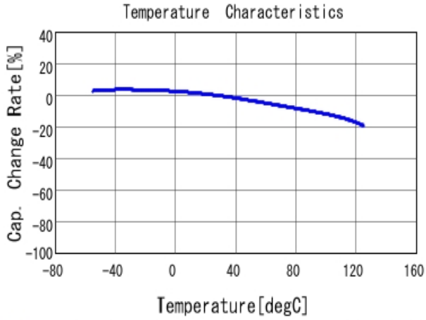
GCM31CC71E106KA03 C-Temp. capchange, DC0.0V, AC1.0V rm
