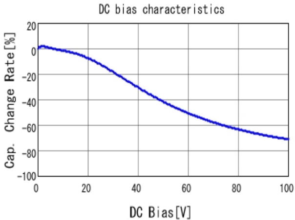
GCM21BR72A104KA37 C-DC bias capchange, 25.0degC, AC1.
