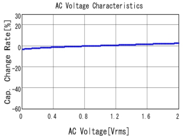
GCM21BR72A104KA37 C-AC Voltage capchange, DCOV, 25.0d
