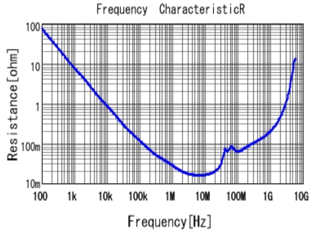
GCM21BR72A104KA37 R DCOV, 25degC
