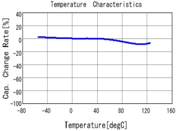
■ GCM21BR72A104KA37 C-Temp. capchange, DC0.0V, AC1.0V r m
