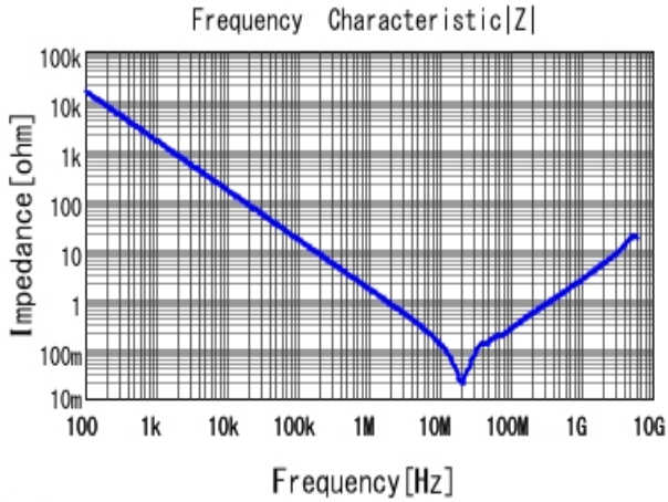
GCM21BR72A104KA37 |Z| DCOV, 25degC
