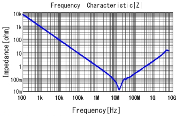
GCM21BR71H224KA37 |Z| DCOV, 25degC
