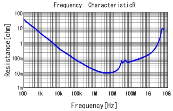
GCM21BR71H224KA37 R DCOV, 25degC
