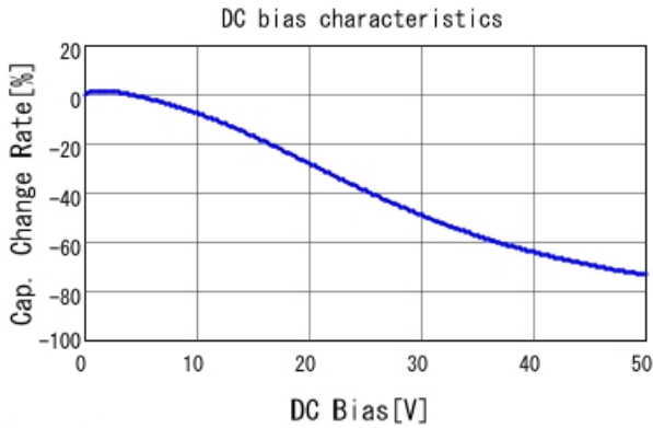
GCM21BR71H105KA03 C-DC bias capchange, 25.0degC, A
