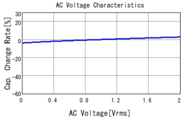
GCM21BR71H105KA03 C-AC Voltage capchange, DCOV, 25
