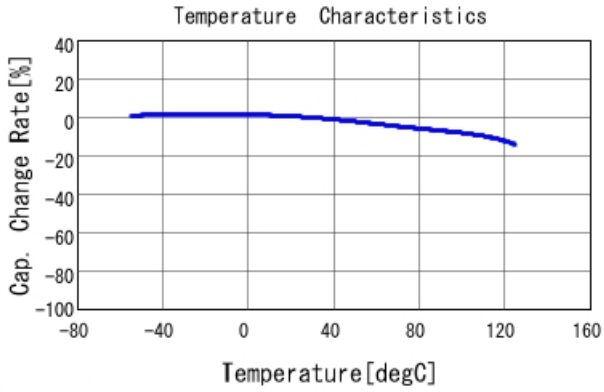
GCM21BR71H105KA03 C-Temp. capchange, DC0.0V, AC1.C
