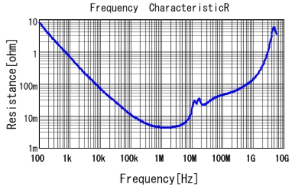
GCM21BR71H105KA03 R DC0V, 25degC
