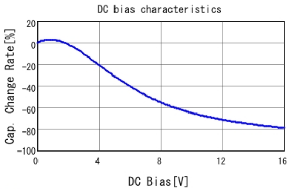
GCM21BR71C475KA73 C-DC bias capchange, 25.0degC, AC1.
