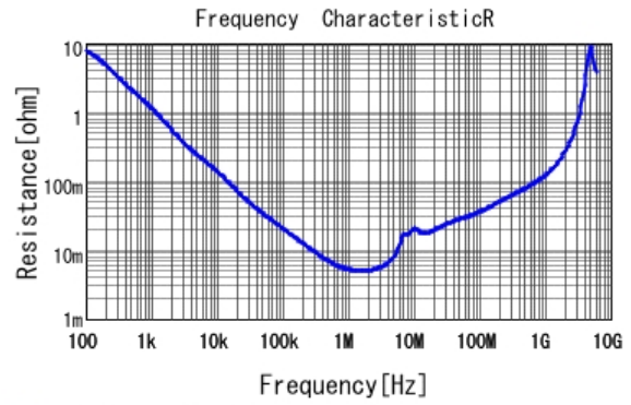
GCM21BR71C475KA73 R DC0V, 25degC
