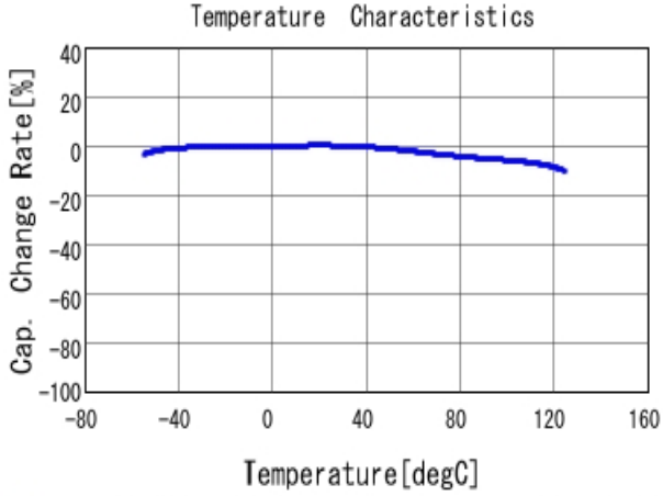
■ GCM21BC72A105KE36 C-Temp. capchange, DC0.0V, AC1.0V r m
