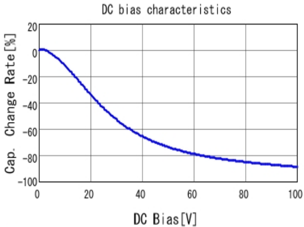
GCM21BC72A105KE36 C-DC bias capchange, 25.0degC, AC1.
