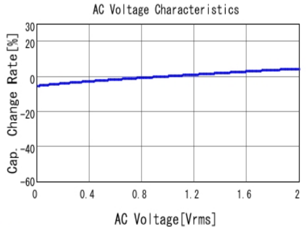
GCM21BC72A105KE36 C-AC Voltage capchange, DCOV, 25.0d
