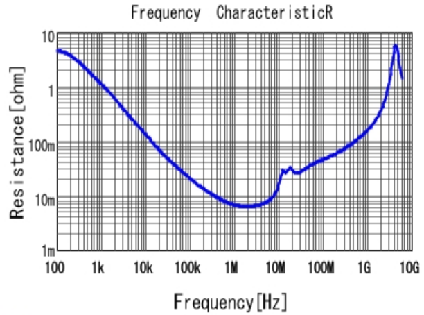
GCM21BC72A105KE36 R DCOV, 25degC
