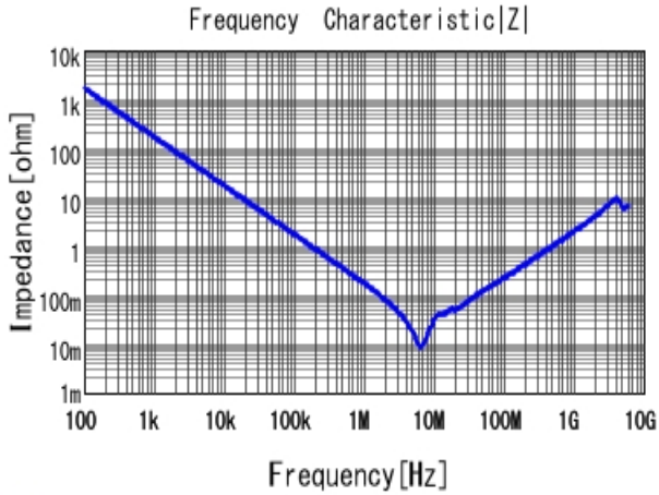
GCM21BC72A105KE36 |Z| DCOV, 25degC
