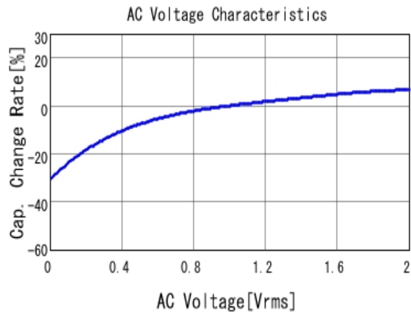
■ GCM21BC71C106KE36 C-AC Voltage capchange, DCOV, 25.0d
