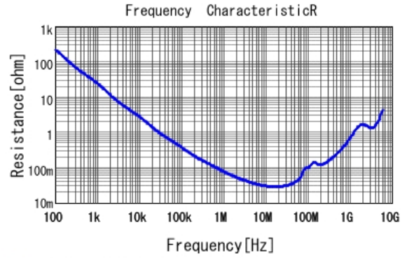
GCM219R72A333KA37 R DCOV, 25degC
