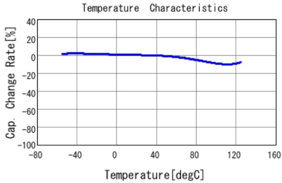
■ GCM219R72A333KA37 C-Temp. capchange, DC0.0V, AC1.0Vrm
