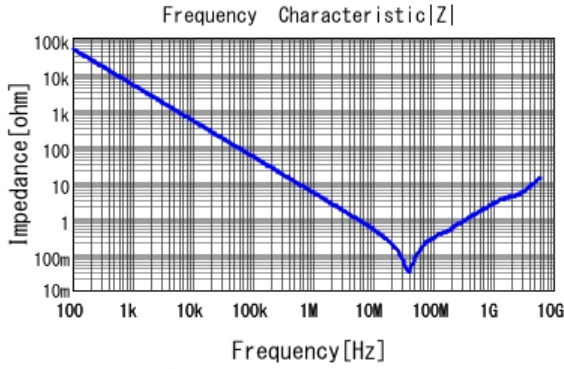
GCM219R72A333KA37 |Z| DCOV, 25degC
