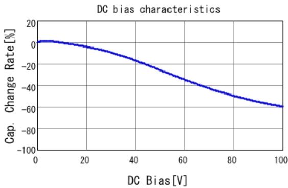
GCM219R72A333KA37 C-DC bias capchange, 25.0degC, AC1.
