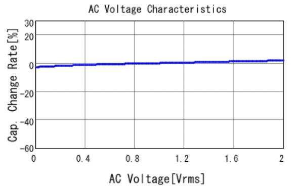
GCM219R72A333KA37 C-AC Voltage capchange, DCOV, 25.0d
