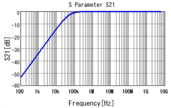
■ GCM219R72A333KA37 S21 DC0V, 25degC
