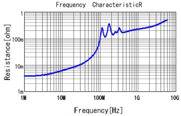
GCM2195C1H153JA16 R DCOV, 25degC
