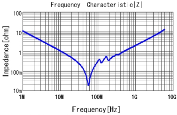
GCM2195C1H153JA16 |Z| DCOV, 25degC
