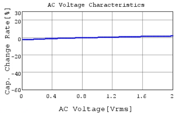
GCM188R72A472KA37 C-AC Voltage capchange, DC
