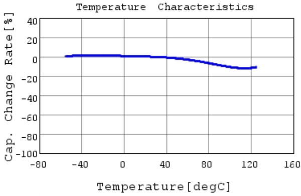
GCM188R72A472KA37 C-Temp. capchange, DC0.0V,
