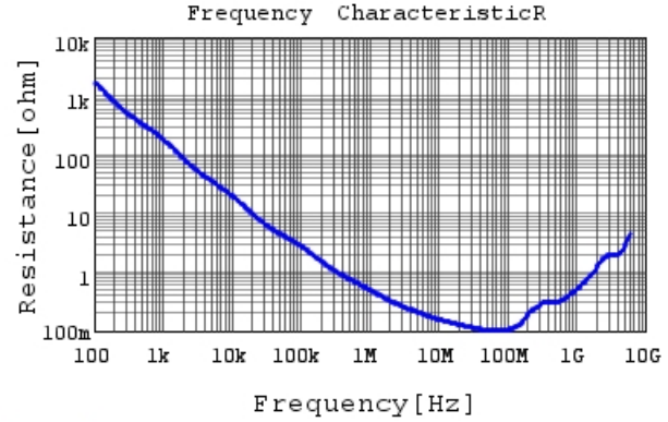
GCM188R72A472KA37 R DC0V, 25degC
