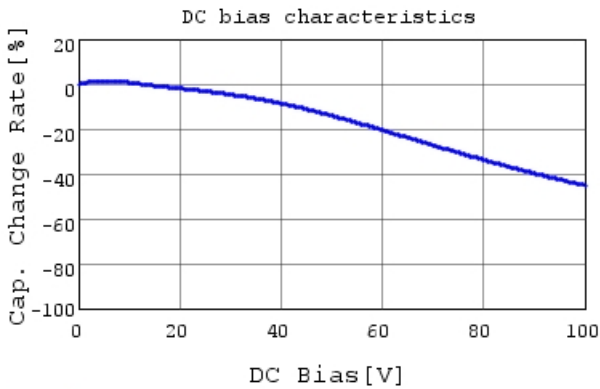
GCM188R72A472KA37 C-DC bias capchange, 25.0c
