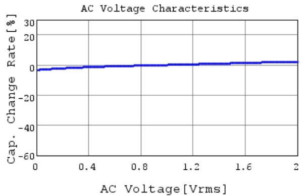
GCM188R72A223KA37 C-AC Voltage capchange, Dc
