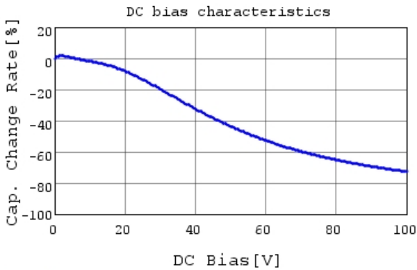
GCM188R72A223KA37 C-DC bias capchange, 25.0c
