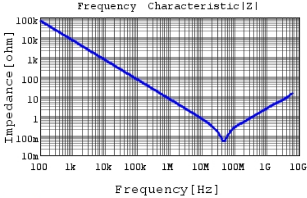
GCM188R72A223KA37 |Z| DCOV, 25degC
