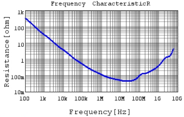
GCM188R72A223KA37 R DCOV, 25degC
