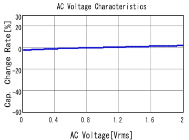
GCM188R72A153KA37 C-AC Voltage capchange, DCOV, 25.0d
