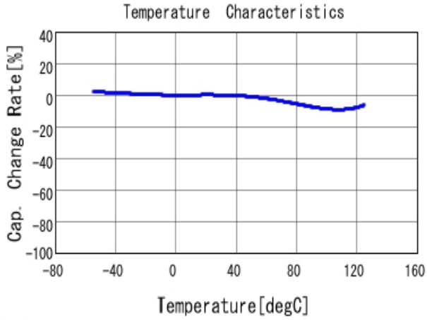
■ GCM188R72A153KA37 C-Temp. capchange, DC0.0V, AC1.0V rm
