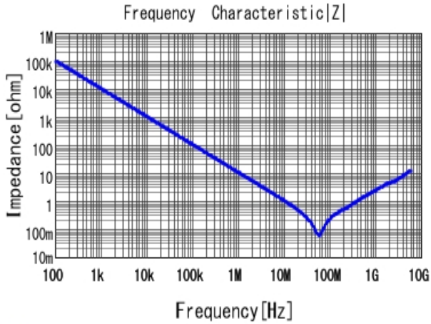
GCM188R72A153KA37 |Z| DCOV, 25degC
