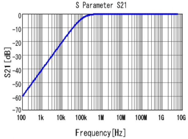
■ GCM188R72A153KA37 S21 DC0V, 25degC
