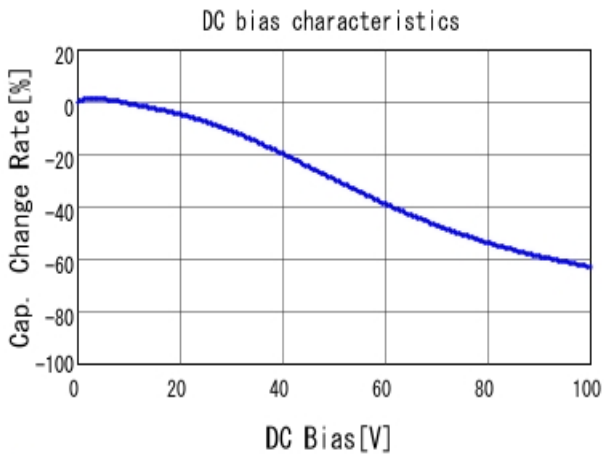
GCM188R72A153KA37 C-DC bias capchange, 25.0degC, AC1.
