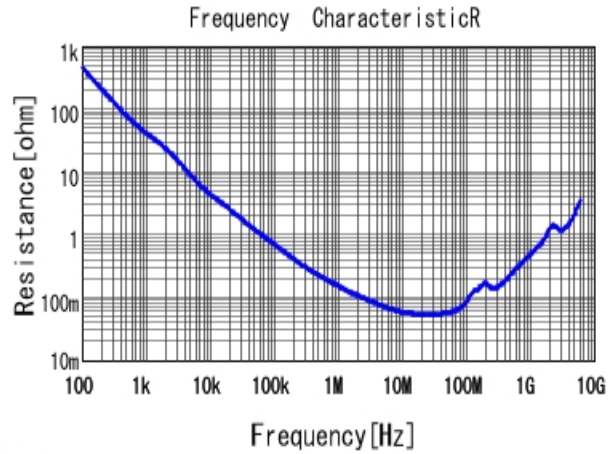
GCM188R72A153KA37 R DCOV, 25degC
