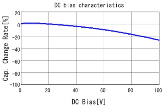
GCM188R72A102KA37 C-DC bias capchange, 25.0degC, AC1.
