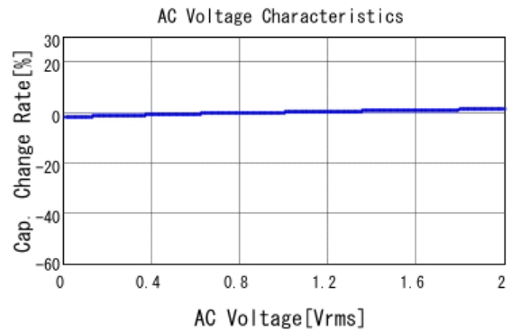
GCM188R72A102KA37 C-AC Voltage capchange, DCOV, 25.0d
