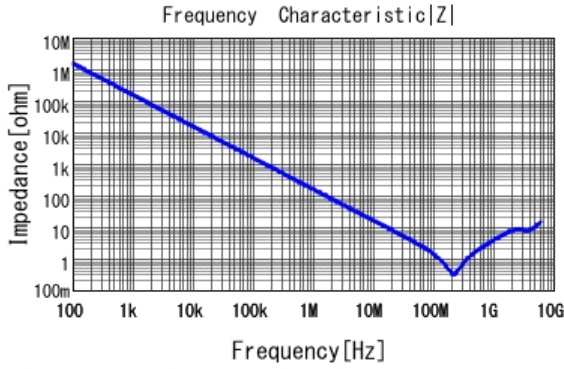
GCM188R72A102KA37 |Z| DCOV, 25degC
