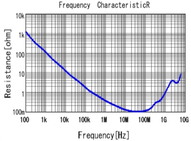
GCM188R71H682KA37 R DCOV, 25degC
