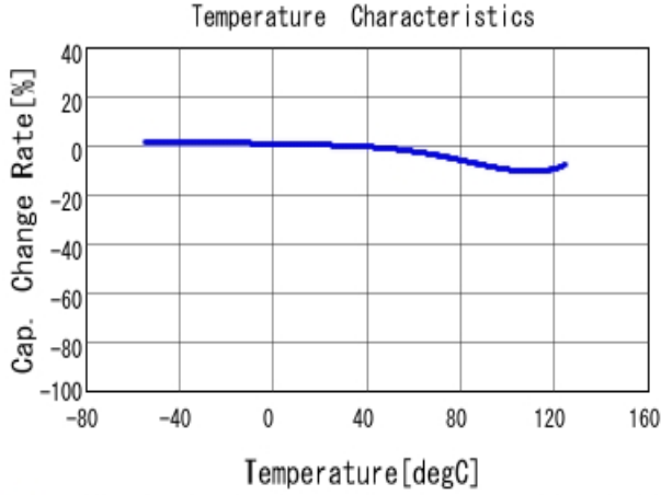
■ GCM188R71H682KA37 C-Temp. capchange, DCO. 0V, AC1.0Vrm
