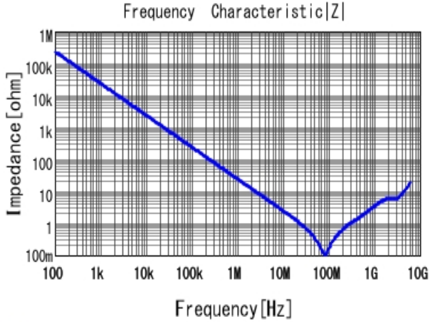
GCM188R71H682KA37 |Z| DCOV, 25degC
