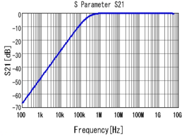
■ GCM188R71H682KA37 S21 DCOV, 25degC
