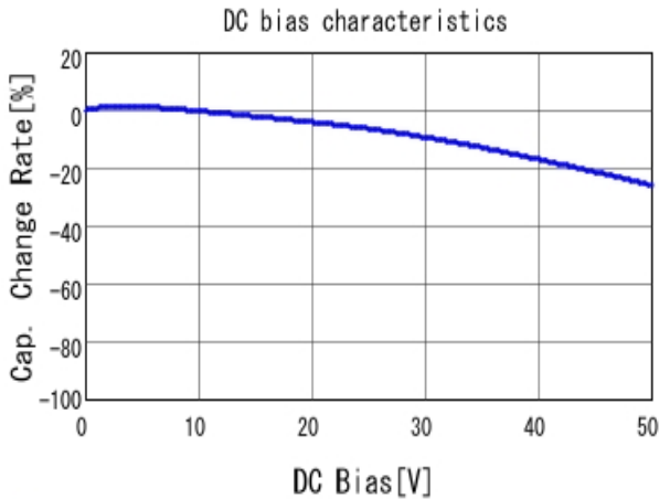
GCM188R71H682KA37 C-DC bias capchange, 25.0degC, AC1.
