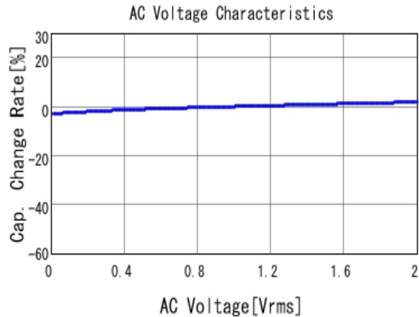
GCM188R71H682KA37 C-AC Voltage capchange, DCOV, 25.0d
