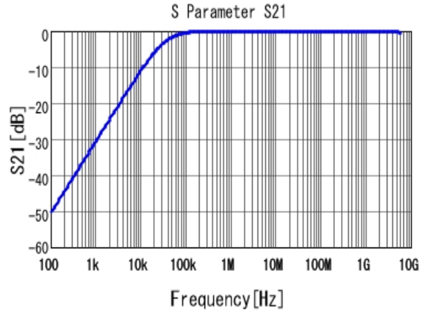
■ GCM188R71H473KA55 S21 DC0V, 25degC
