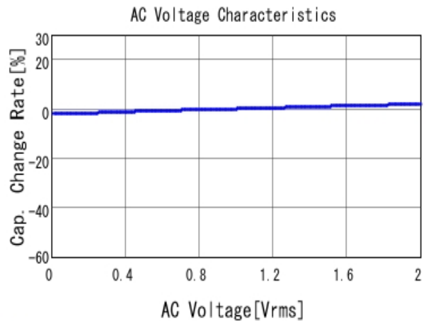
GCM188R71H473KA55 C-AC Voltage capchange, DCOV, 25.0d
