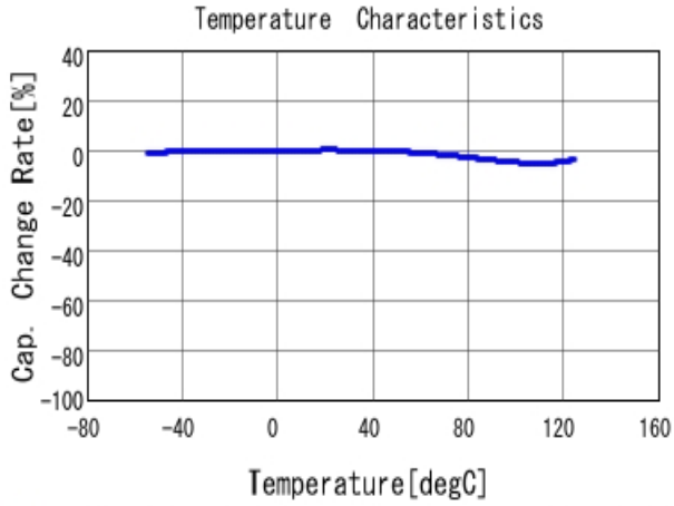
■ GCM188R71H473KA55 C-Temp. capchange, DC0.0V, AC1.0Vrm
