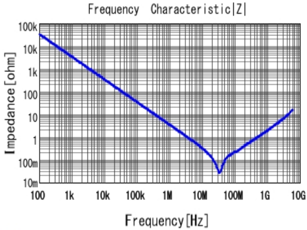
GCM188R71H473KA55 |Z| DCOV, 25degC
