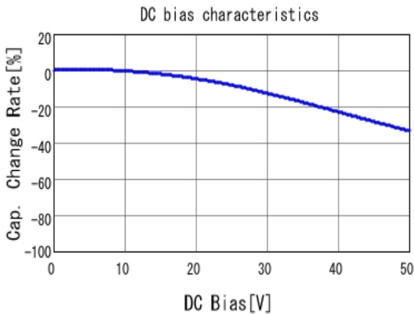
GCM188R71H473KA55 C-DC bias capchange, 25.0degC, AC1.
