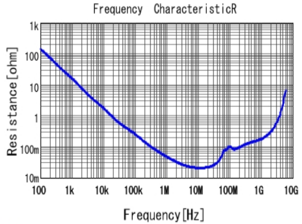
GCM188R71H473KA55 R DCOV, 25degC
