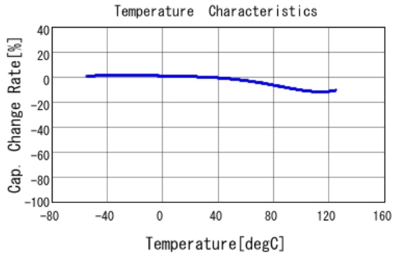
■ GCM188R71H472KA37 C-Temp. capchange, DC0.0V, AC1.0V r m
