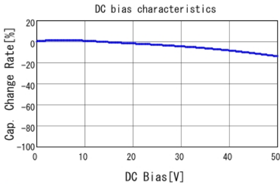
GCM188R71H472KA37 C-DC bias capchange, 25.0degC, AC1.
