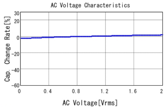
GCM188R71H472KA37 C-AC Voltage capchange, DCOV, 25.0d
