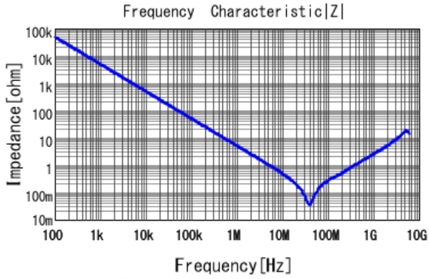
GCM188R71H333KA55 |Z| DCOV, 25degC
