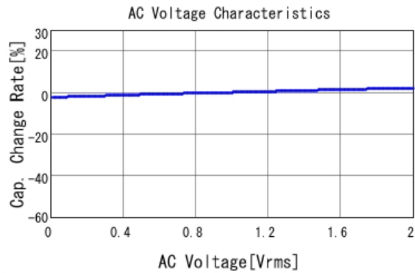
GCM188R71H333KA55 C-AC Voltage capchange, DCOV, 25
