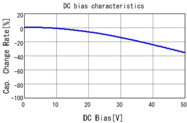
GCM188R71H333KA55 C-DC bias capchange, 25.0degC, A
