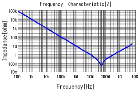
■ GCM188R71H223KA37 |Z| DCOV, 25degC
