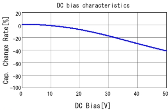
■ GCM188R71H223KA37 C-DC bias capchange, 25.0degC, AC1.
