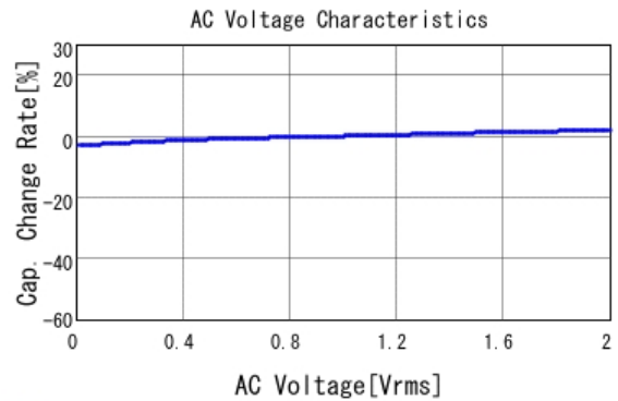
■ GCM188R71H223KA37 C-AC Voltage capchange, DCOV, 25.0d
