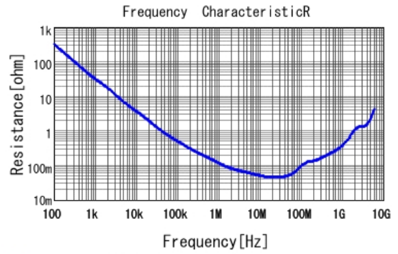
■ GCM188R71H223KA37 R DCOV, 25degC
