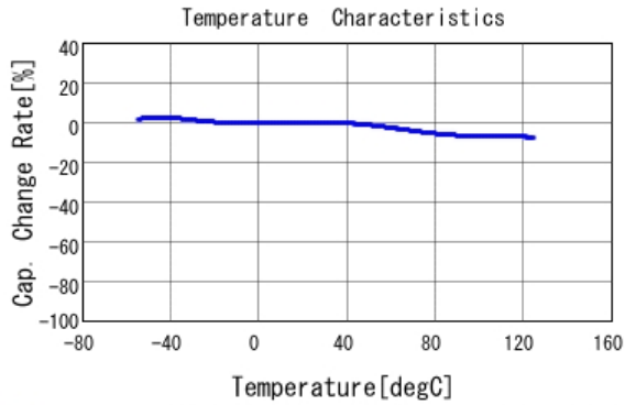
■ GCM188R71H223KA37 C-Temp. capchange, DC0.0V, AC1.0V rm
