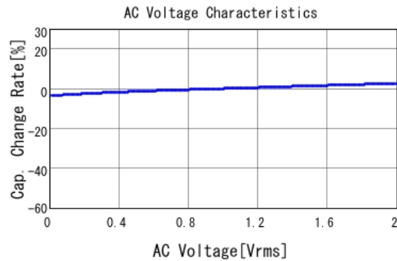
■ GCM188R71H154KA64 C-AC Voltage capchange, DC0V, 25.0d
