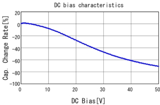
■ GCM188R71H154KA64 C-DC bias capchange, 25.0degC, AC1.
