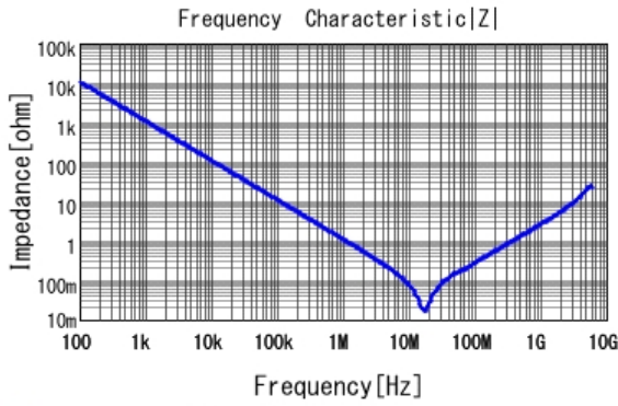
■ GCM188R71H154KA64 |Z| DC0V, 25degC
