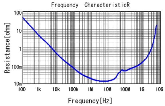
■ GCM188R71H154KA64 R DC0V, 25degC
