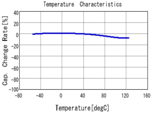
■ GCM188R71H104KA57 C-Temp. capchange, DC0.0V, AC1.0V rm
