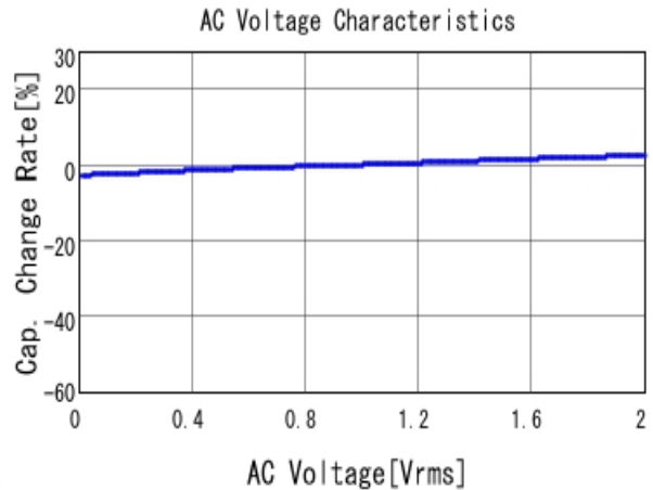
■ GCM188R71H104KA57 C-AC Voltage capchange, DC0V, 25.0d
