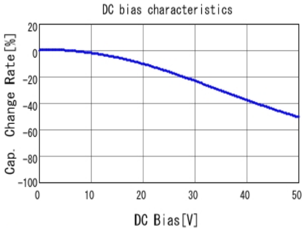
■ GCM188R71H104KA57 C-DC bias capchange, 25.0degC, AC1.
