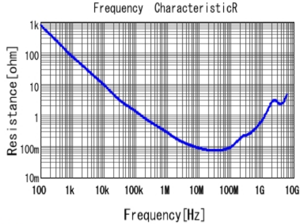
GCM188R71H103KA37 R DCOV, 25degC
