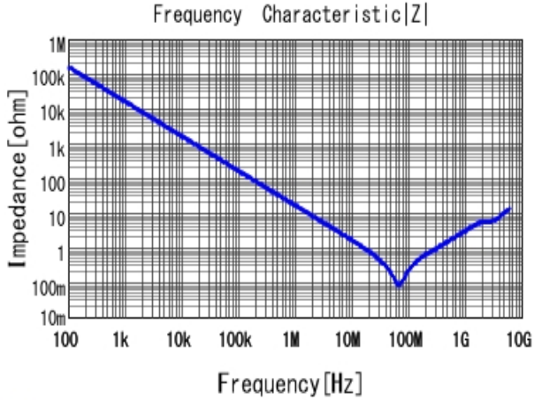
GCM188R71H103KA37 |Z| DCOV, 25degC
