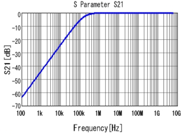
■ GCM188R71H103KA37 S21 DCOV, 25degC
