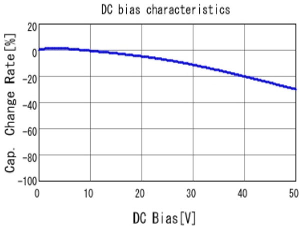
GCM188R71H103KA37 C-DC bias capchange, 25.0degC, AC1.
