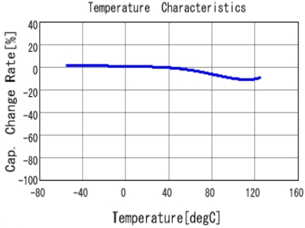
■ GCM188R71H103KA37 C-Temp. capchange, DCO. 0V, AC1.0V rm
