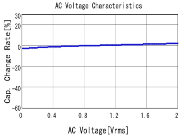
GCM188R71H103KA37 C-AC Voltage capchange, DCOV, 25.0d
