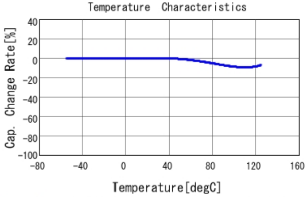
GCM188R71H102KA37 C-Temp. capchange, DC0.0V, AC1.C
