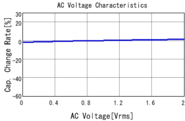
GCM188R71H102KA37 C-AC Voltage capchange, DCOV, 25
