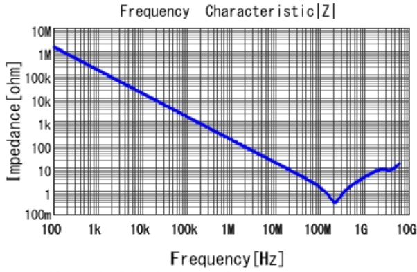
GCM188R71H102KA37 |Z| DCOV, 25degC
