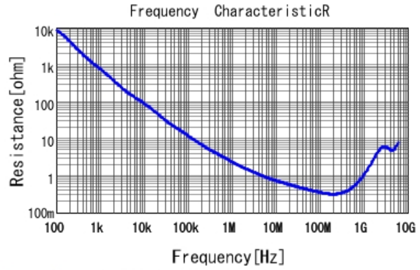
GCM188R71H102KA37 R DCOV, 25degC
