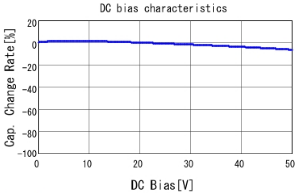
GCM188R71H102KA37 C-DC bias capchange, 25.0degC, A
