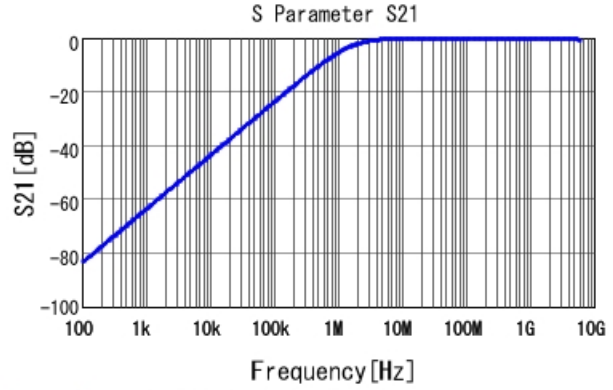
GCM188R71H102KA37 S21 DC0V, 25degC
