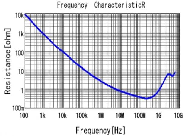
GCM188R71H102KA37 R DCOV, 25degC
