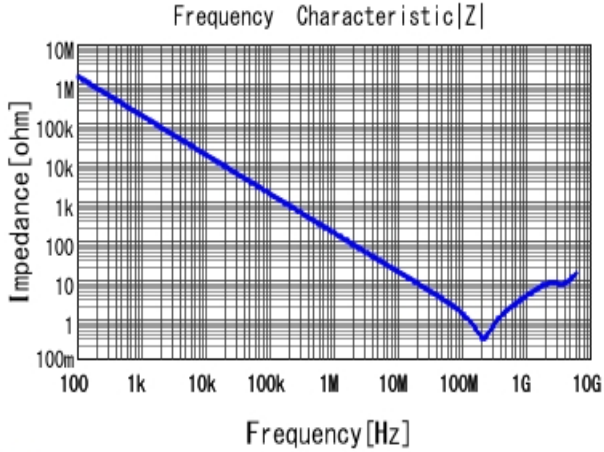
GCM188R71H102KA37 |Z| DCOV, 25degC
