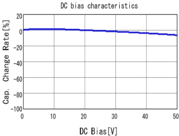
GCM188R71H102KA37 C-DC bias capchange, 25.0degC, AC1.
