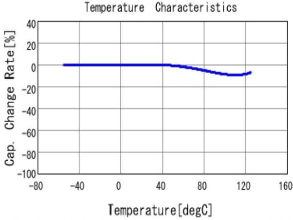
■ GCM188R71H102KA37 C-Temp. capchange, DCO. 0V, AC1.0Vrm
