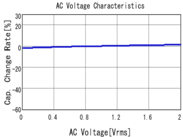
GCM188R71H102KA37 C-AC Voltage capchange, DCOV, 25.0d
