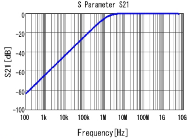
■ GCM188R71H102KA37 S21 DCOV, 25degC
