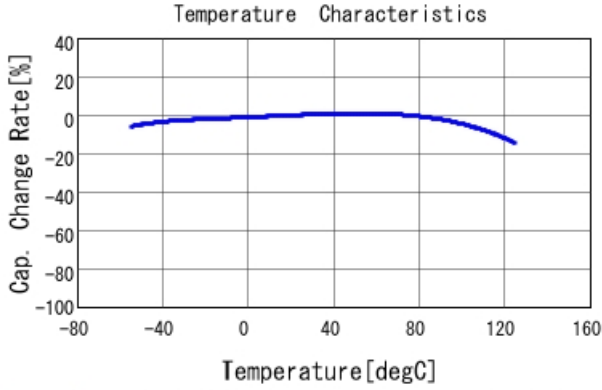
GCM188R71E105KA64 C-Temp. capchange, DC0.0V, AC1.C
