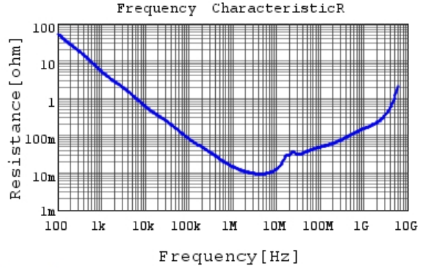
GCM188R71E105KA64 R DCOV, 25degC
