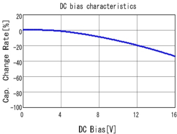
GCM188R71C334KA37 C-DC bias capchange, 25.0degC, AC1.
