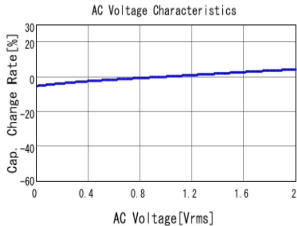
GCM188R71C334KA37 C-AC Voltage capchange, DCOV, 25.0d
