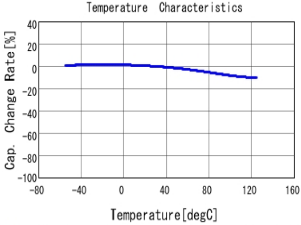
GCM188R71C334KA37 C-Temp. capchange, DC0.0V, AC1.0V rm
