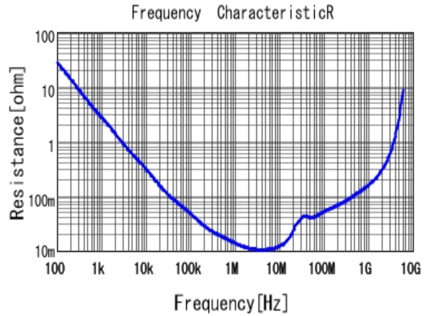
GCM188R71C334KA37 R DCOV, 25degC
