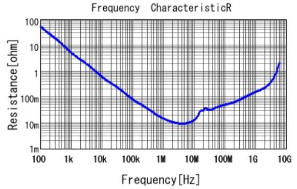
GCM188R71C105KA64 R DC0V, 25degC
