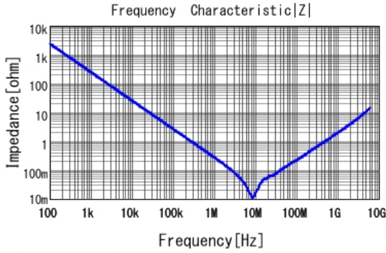
GCM188R71C105KA64 |Z| DC0V, 25degC
