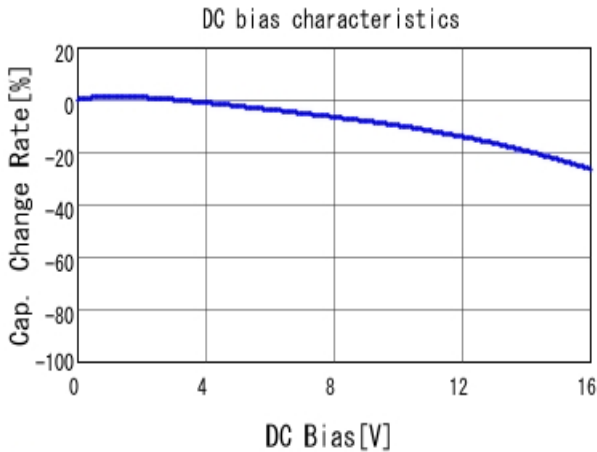
GCM188R71C104KA37 C-DC bias capchange, 25.0degC, AC1.
