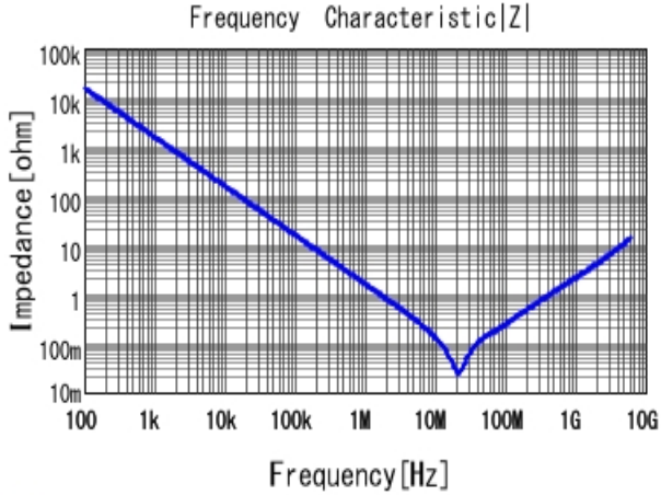
GCM188R71C104KA37 |Z| DCOV, 25degC
