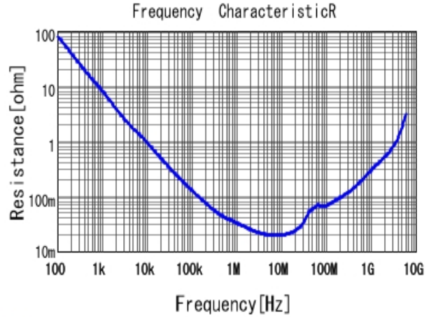
GCM188R71C104KA37 R DCOV, 25degC
