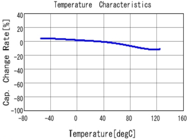
GCM188R71C104KA37 C-Temp. capchange, DC0.0V, AC1.0V rm
