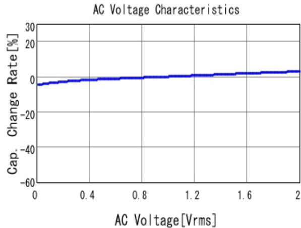
GCM188R71C104KA37 C-AC Voltage capchange, DCOV, 25.0d
