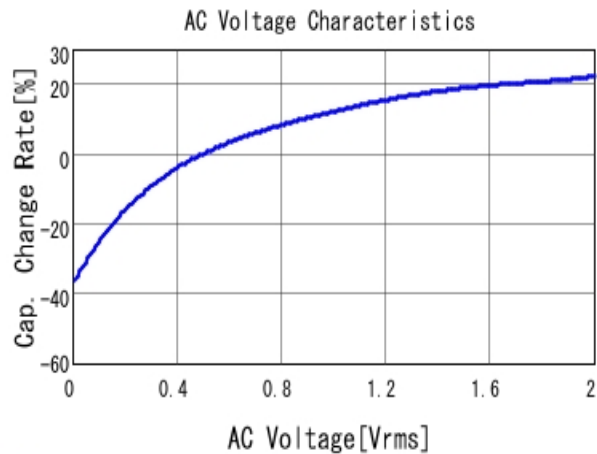
GCM188R70J225KE22 C-AC Voltage capchange, DCOV, 25.0d
