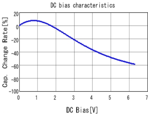
GCM188R70J225KE22 C-DC bias capchange, 25.0degC, AC0.
