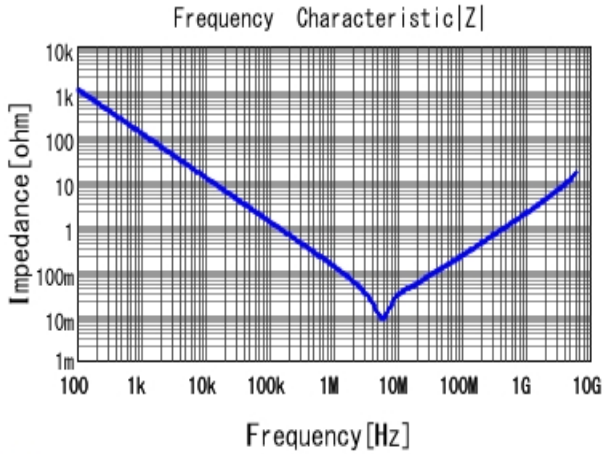
GCM188R70J225KE22 |Z| DCOV, 25degC
