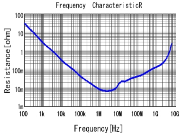
GCM188R70J225KE22 R DCOV, 25degC
