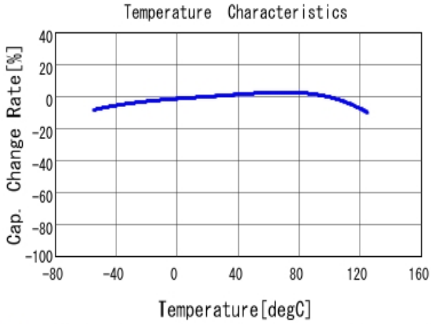
GCM188R70J225KE22 C-Temp. capchange, DCO. 0V, ACO. 5V rm
