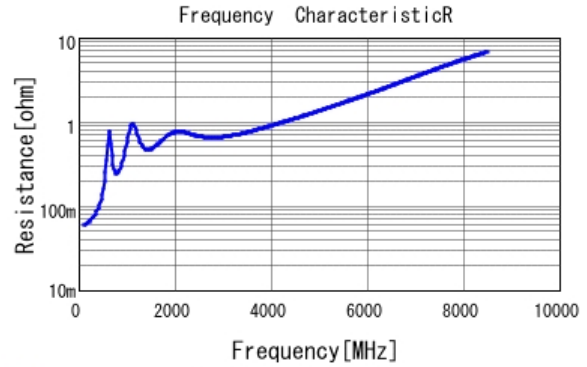
■ GCM1885C2A471JA16 R DC0V, 25degC
