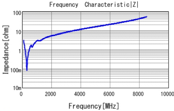
■ GCM1885C2A471JA16 |Z| DC0V, 25degC
