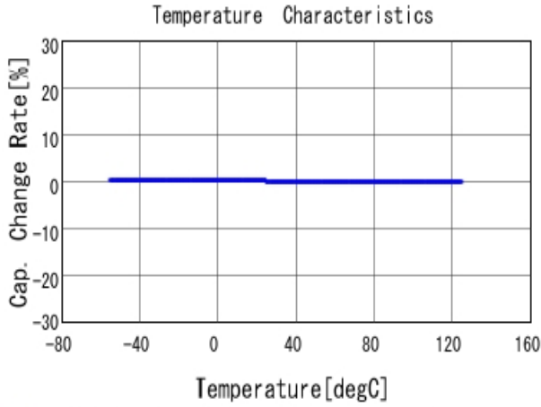
■ GCM1885C2A330JA16 C-Temp. capchange, DCOV, AC1Vrms
