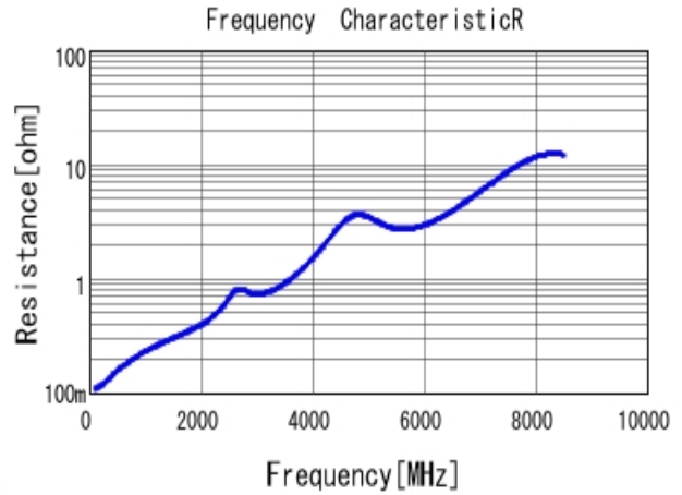
■ GCM1885C2A330JA16 R DC0V, 25degC
