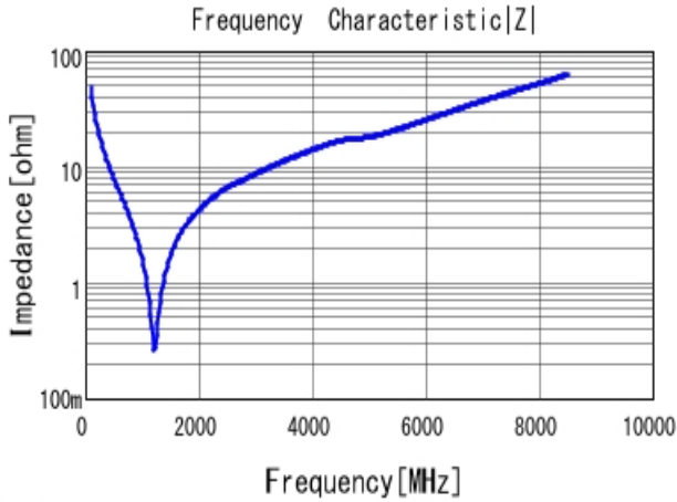
■ GCM1885C2A330JA16 |Z| DC0V, 25degC
