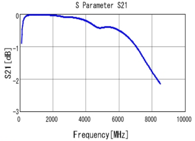
■ GCM1885C2A330JA16 S21 DCOV, 25degC
