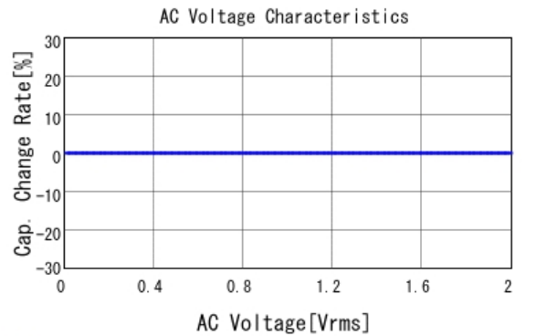
■ GCM1885C2A220JA16 C-AC Voltage capchange, DCOV, 25.0d
