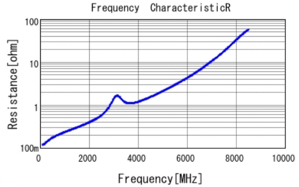
■ GCM1885C2A220JA16 R DCOV, 25degC
