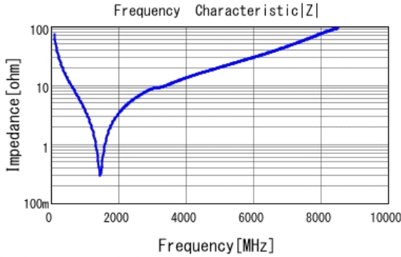
■ GCM1885C2A220JA16 |Z| DCOV, 25degC
