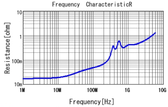
■ GCM1885C2A152JA16 R DCOV, 25degC
