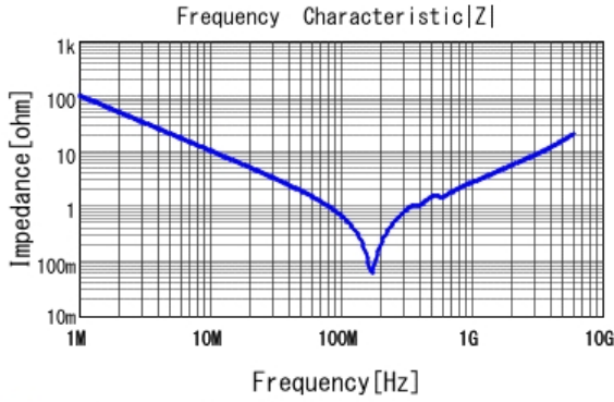
■ GCM1885C2A152JA16 |Z| DCOV, 25degC
