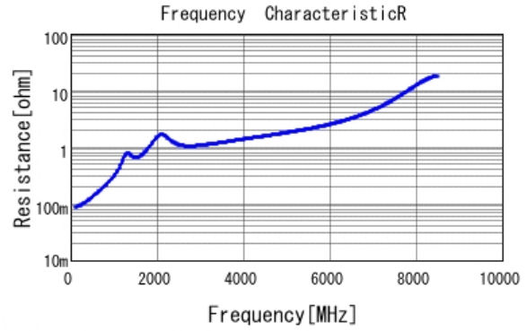
■ GCM1885C2A151JA16 R DCOV, 25degC
