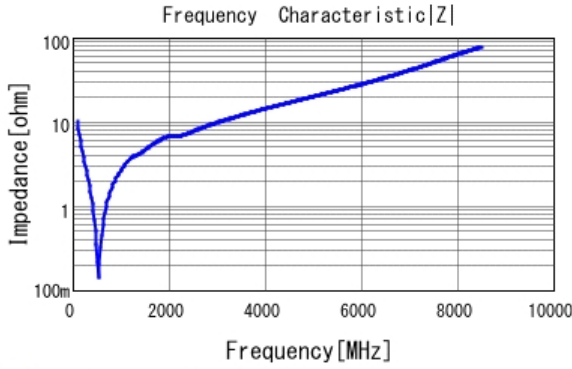
■ GCM1885C2A151JA16 |Z| DCOV, 25degC
