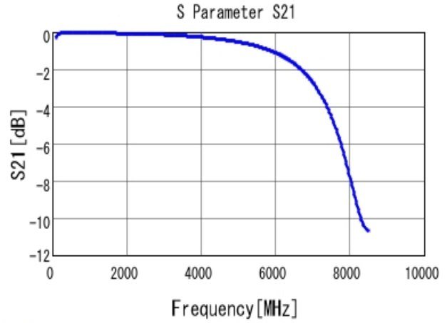
■ GCM1885C1H560JA16 S21 DCOV, 25degC
