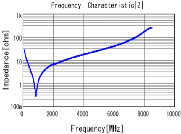
GCM1885C1H560JA16 |Z| DC0V, 25degC
