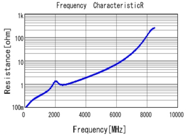
GCM1885C1H560JA16 R DC0V, 25degC
