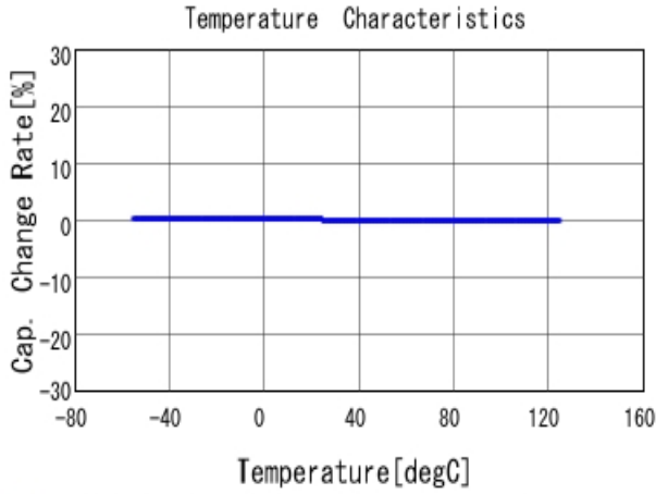
■ GCM1885C1H560JA16 C-Temp. capchange, DCOV, AC1Vrms
