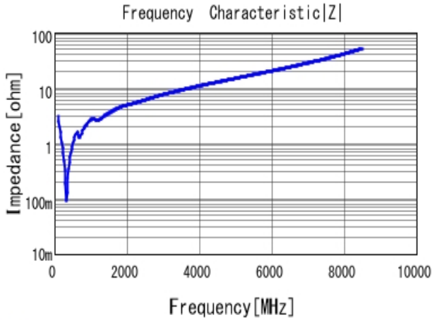
GCM1885C1H471JA16 |Z| DC0V, 25degC
