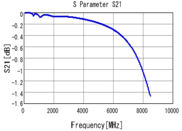
■ GCM1885C1H471JA16 S21 DCOV, 25degC
