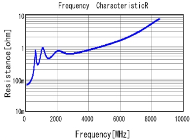
GCM1885C1H471JA16 R DC0V, 25degC
