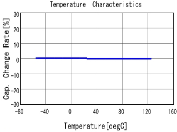
■ GCM1885C1H471JA16 C-Temp. capchange, DCOV, AC1Vrms
