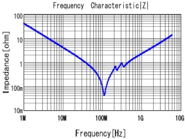
GCM1885C1H392JA16 |Z| DCOV, 25degC
