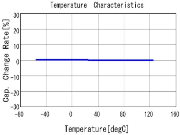
■ GCM1885C1H392JA16 C-Temp. capchange, DCOV, AC1Vrms
