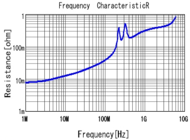
GCM1885C1H392JA16 R DCOV, 25degC
