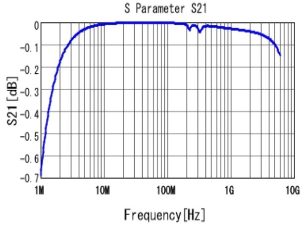
■ GCM1885C1H392JA16 S21 DCOV, 25degC
