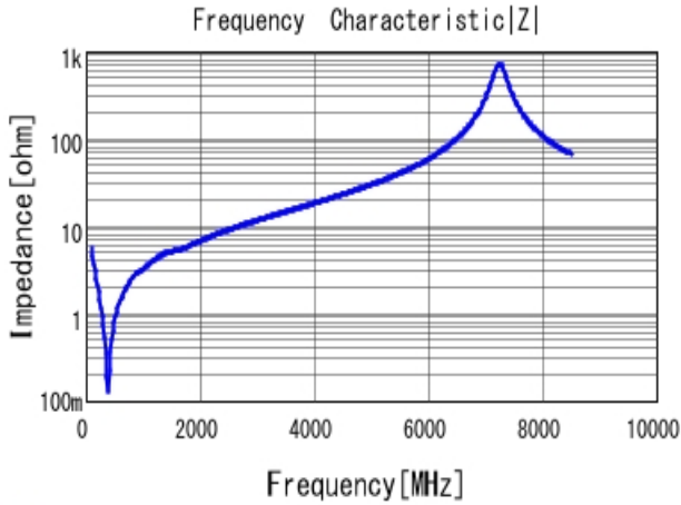
GCM1885C1H271JA16 |Z| DC0V, 25degC
