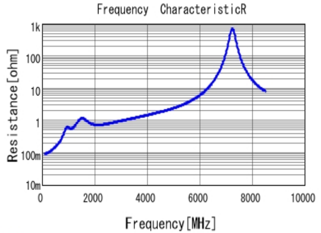
GCM1885C1H271JA16 R DC0V, 25degC
