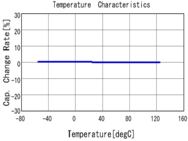
■ GCM1885C1H271JA16 C-Temp. capchange, DCOV, AC1Vrms
