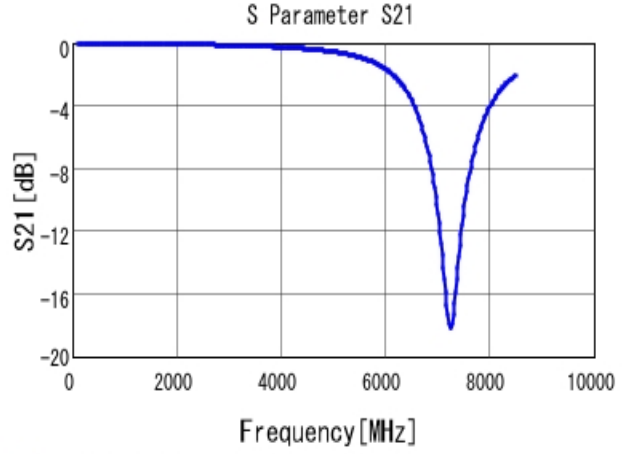
■ GCM1885C1H271JA16 S21 DCOV, 25degC
