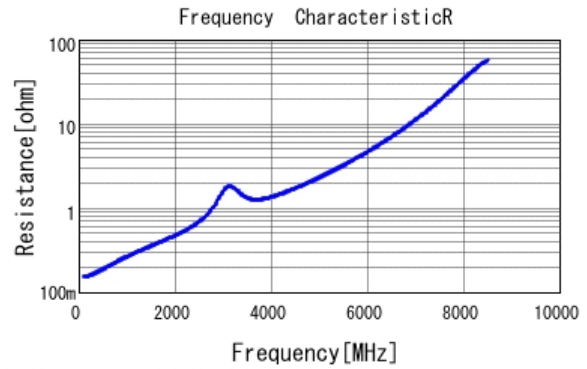
■ GCM1885C1H220JA16 R DCOV, 25degC
