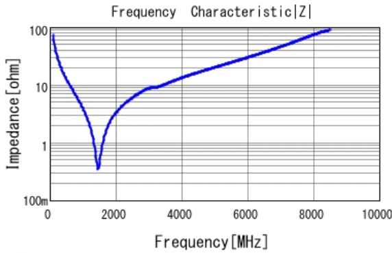
■ GCM1885C1H220JA16 |Z| DCOV, 25degC
