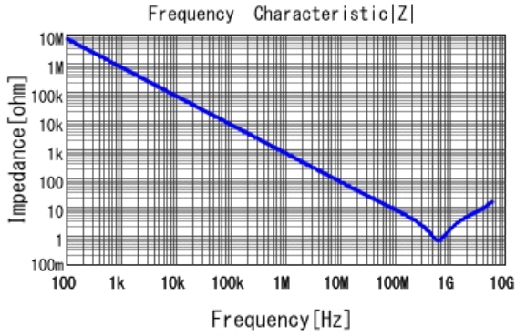
GCM155R72A221KA37 |Z| DCOV, 25degC
