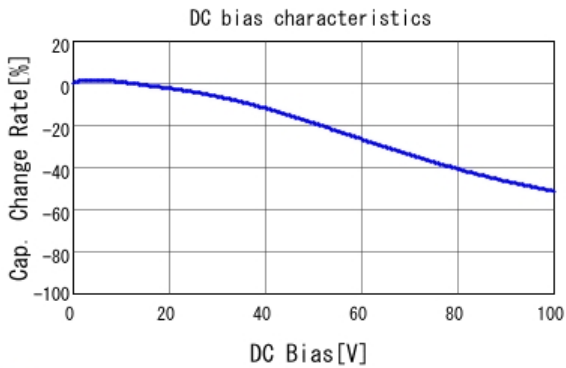
GCM155R72A221KA37 C-DC bias capchange, 25.0degC, AC1.
