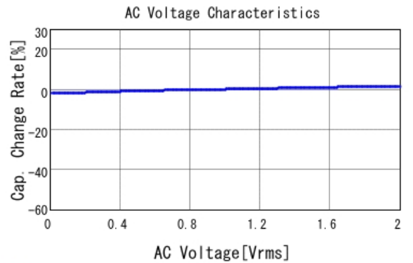
GCM155R72A221KA37 C-AC Voltage capchange, DCOV, 25.0d
