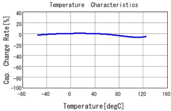
■ GCM155R71H682KA55 C-Temp. capchange, DC0.0V, AC1.0V rm
