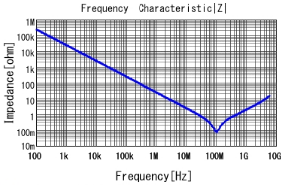
GCM155R71H682KA55 |Z| DCOV, 25degC
