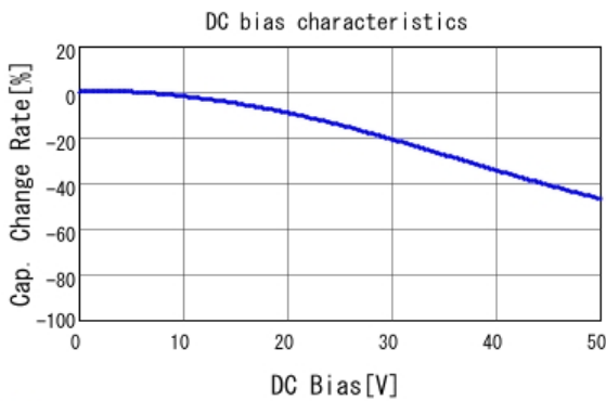
GCM155R71H682KA55 C-DC bias capchange, 25.0degC, AC1.
