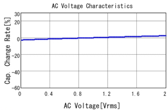
GCM155R71H682KA55 C-AC Voltage capchange, DCOV, 25.0d
