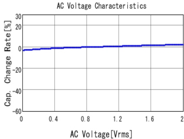
GCM155R71H472KA37 C-AC Voltage capchange, DCOV, 25.0d
