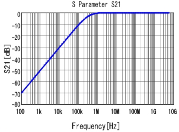
■ GCM155R71H472KA37 S21 DCOV, 25degC
