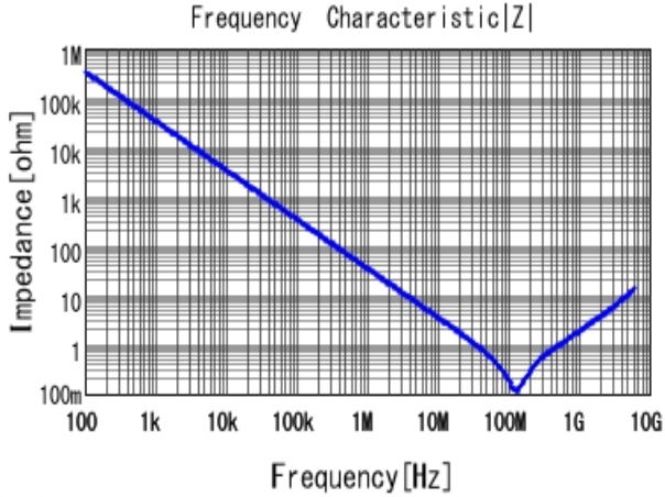
GCM155R71H472KA37 |Z| DCOV, 25degC
