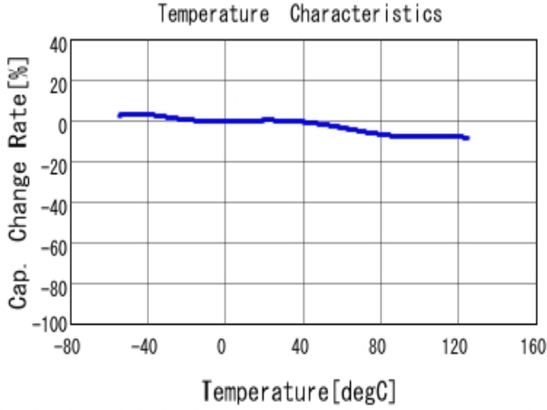
■ GCM155R71H472KA37 C-Temp. capchange, DCO. 0V, AC1.0V rm
