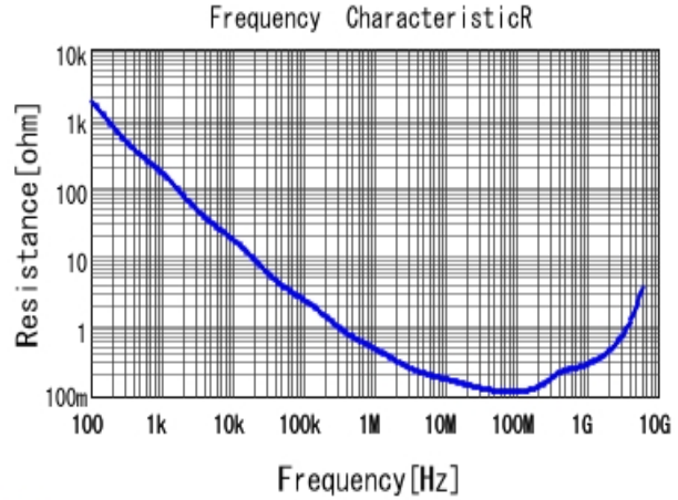
GCM155R71H472KA37 R DCOV, 25degC
