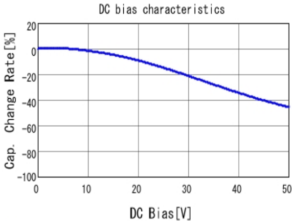
GCM155R71H472KA37 C-DC bias capchange, 25.0degC, AC1.
